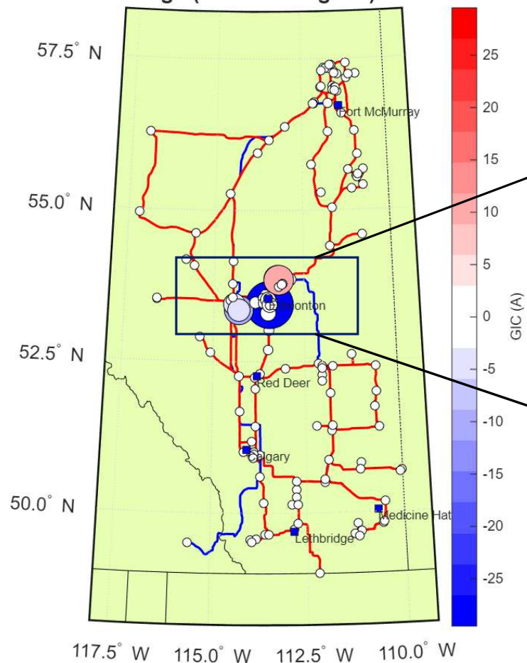
Max GIC Change (Edited - Original) - Full Alberta
